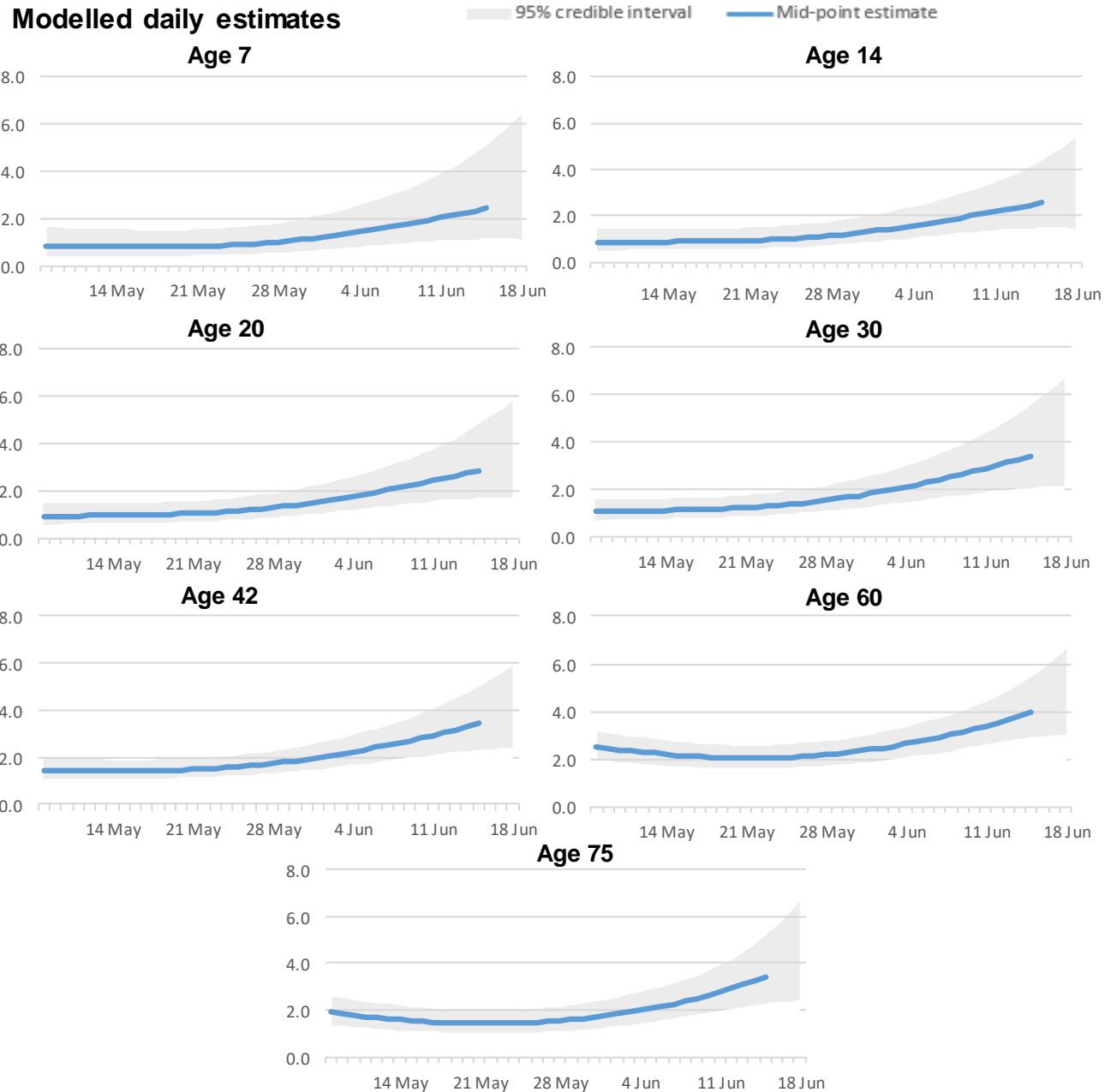
Figure 2 – Percentage of people testing positive for COVID-19 for reference ages in Northern Ireland (Data from 8 May 2022 to 18 June 2022)
