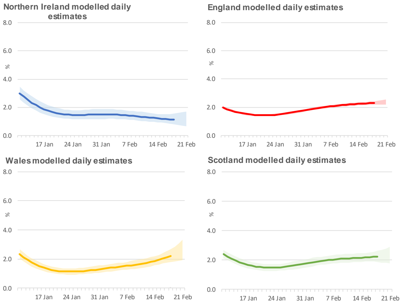
Figure 2: Modelled daily estimate of percentage of the population testing positive for the COVID-19 across the UK
