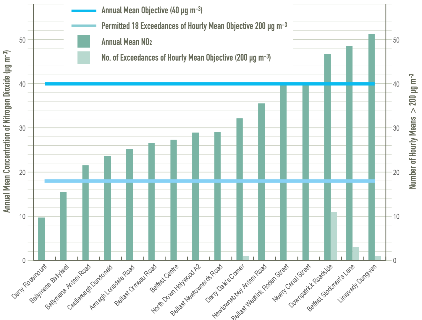
Figure 4.2: Annual Mean NO 2 Concentrations and Exceedances of Hourly Objective, 2018
