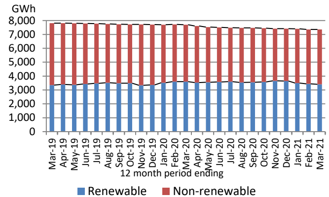
Figure 3: Rolling 12 month Volume of Electricity Consumed by Source (Mar 2019 – Mar 2021)
