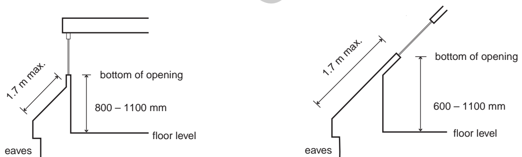
(a) Dormer window
