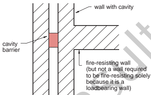
(c) Plan
