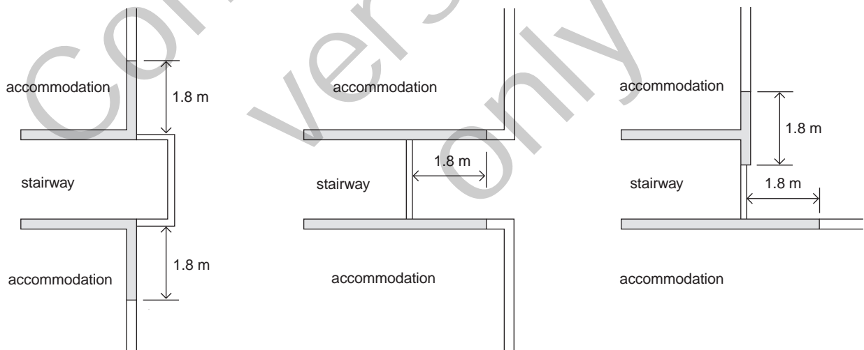
(a) projecting stairway
