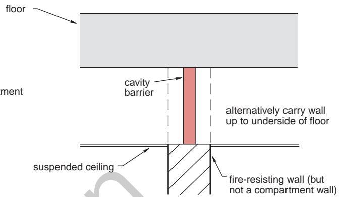
(b) Section
