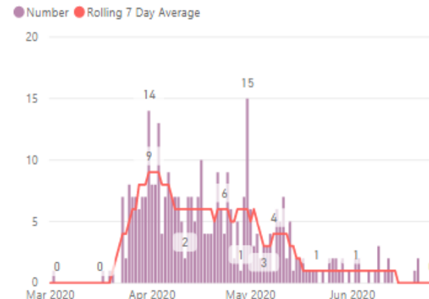
Confirmed COVID-19 daily admissions (Western Trust)
