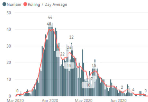
Confirmed COVID-19 daily admissions (South Eastern Trust)
