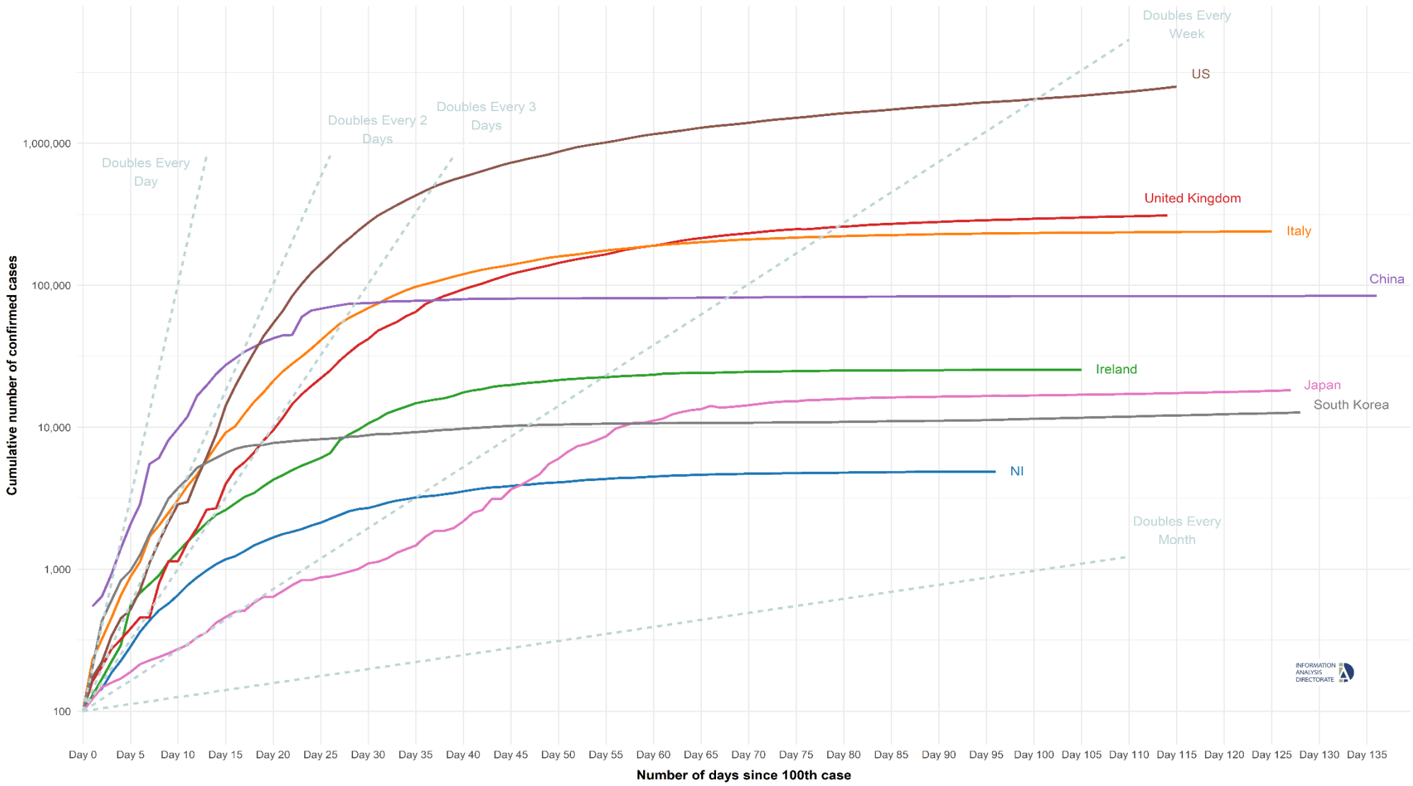
Figure 1: Cumulative number of individuals with a laboratory confirmed test for COVID-19 after the 100 th case. The 100 th case for all countries are aligned by calculating the first time the cumulative number of positive cases was greater than or equal to 100 and rounding down to exactly 100. Data is not available for China before their 500 th case.
