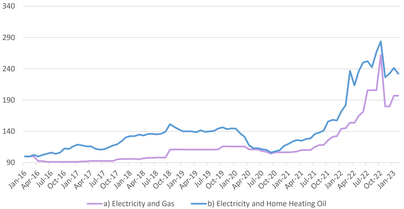
Figure 2: Home Energy Index for (a) Electricity and Gas and (b) Electricity and Home Heating Oil for Northern Ireland (January 2016 – February 2023).
