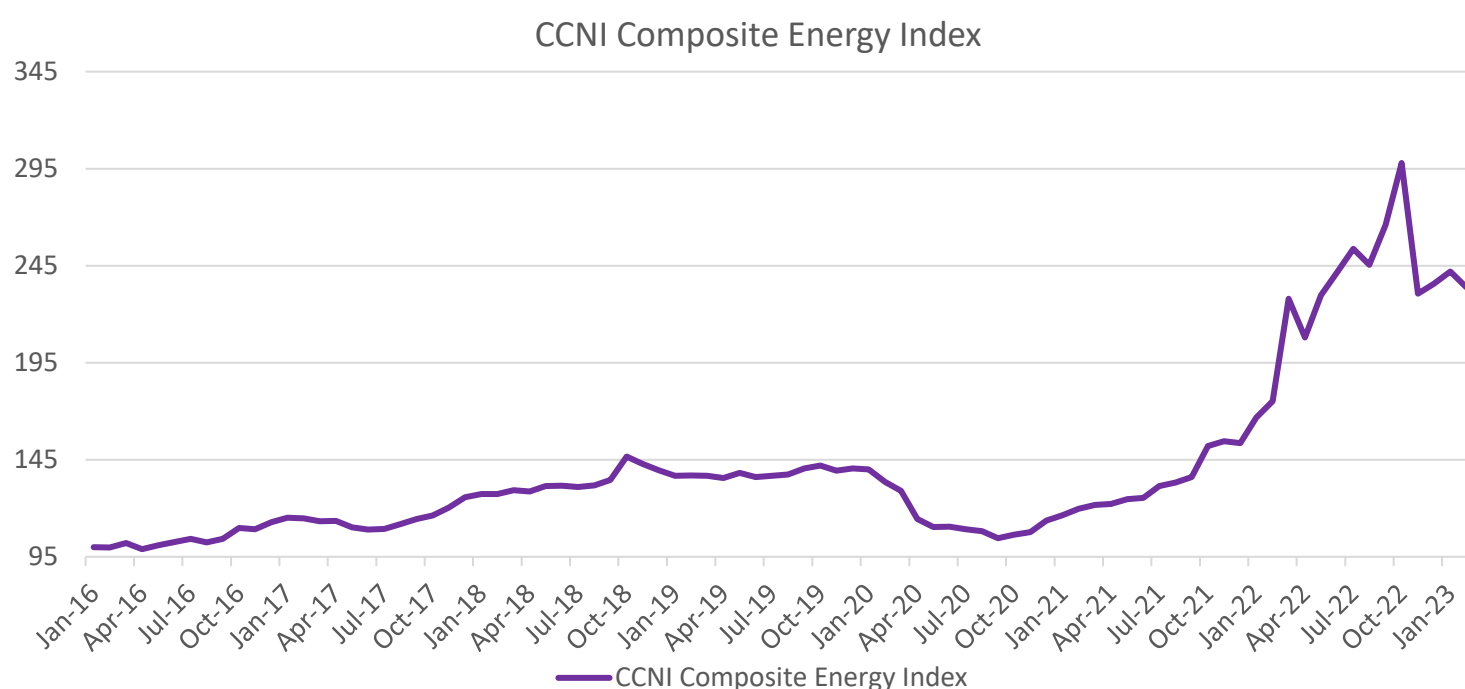
Figure 1: Home Energy Index (composite of electricity, gas and HHO) for Northern Ireland (January 2016 – February 2023). *Incorporating the EPG
