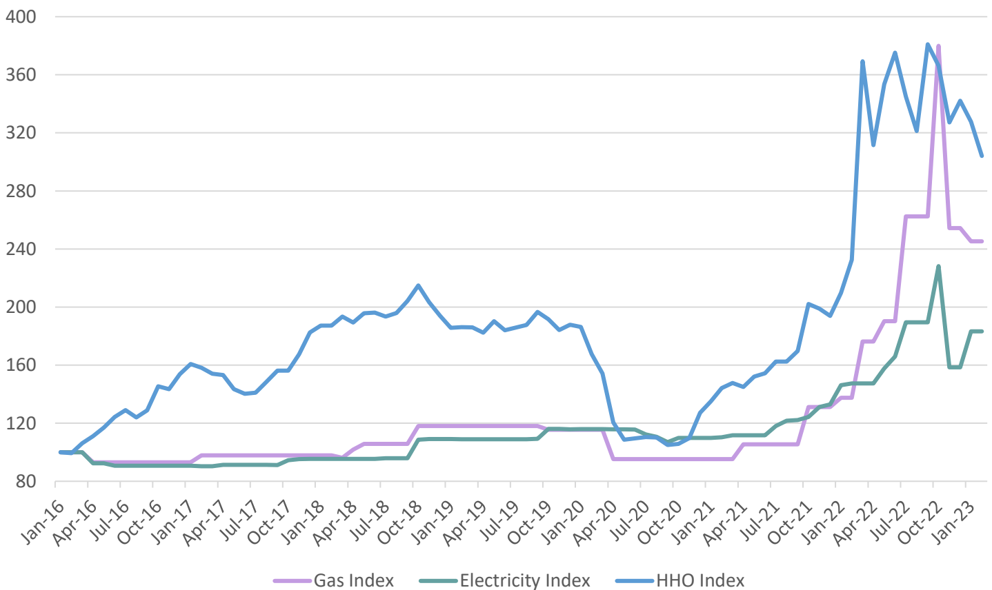
Figure 3: Gas, electricity and home heating oil (HHO) indices for Northern Ireland (January 2016 – February 2023).
