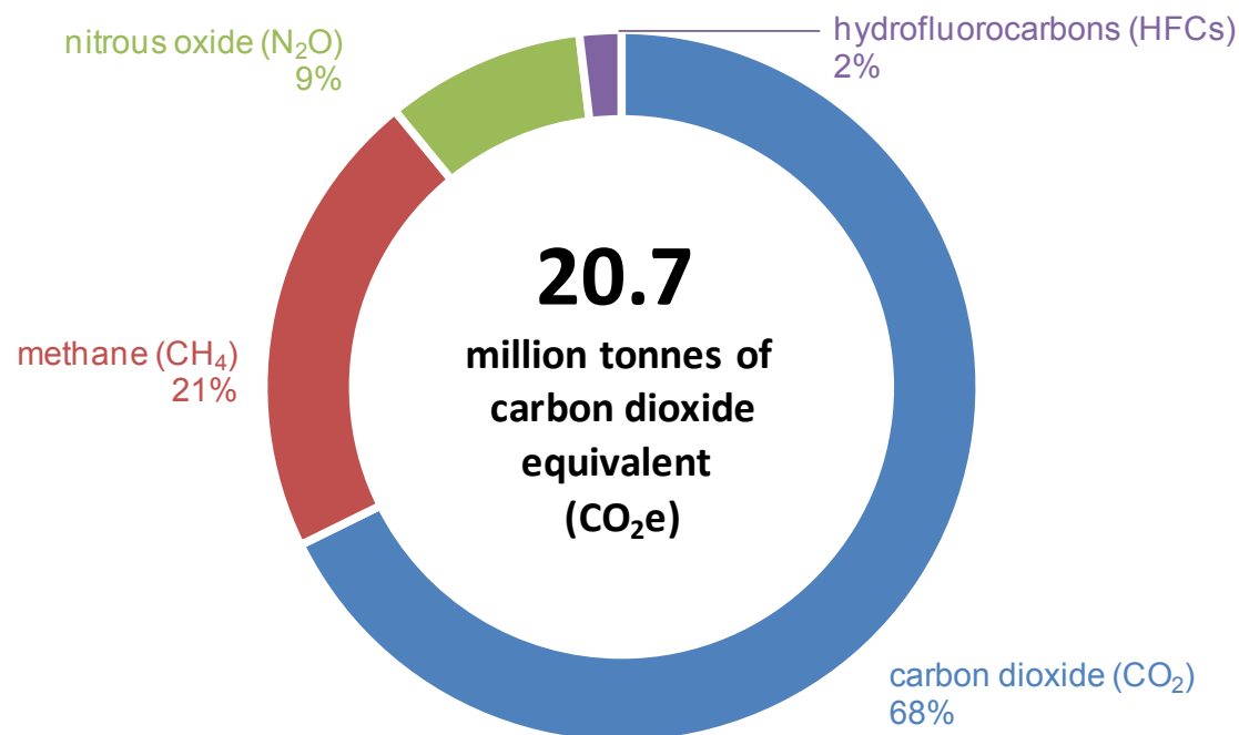
Figure 1: Greenhouse gas emissions by gas Northern Ireland, 2015
