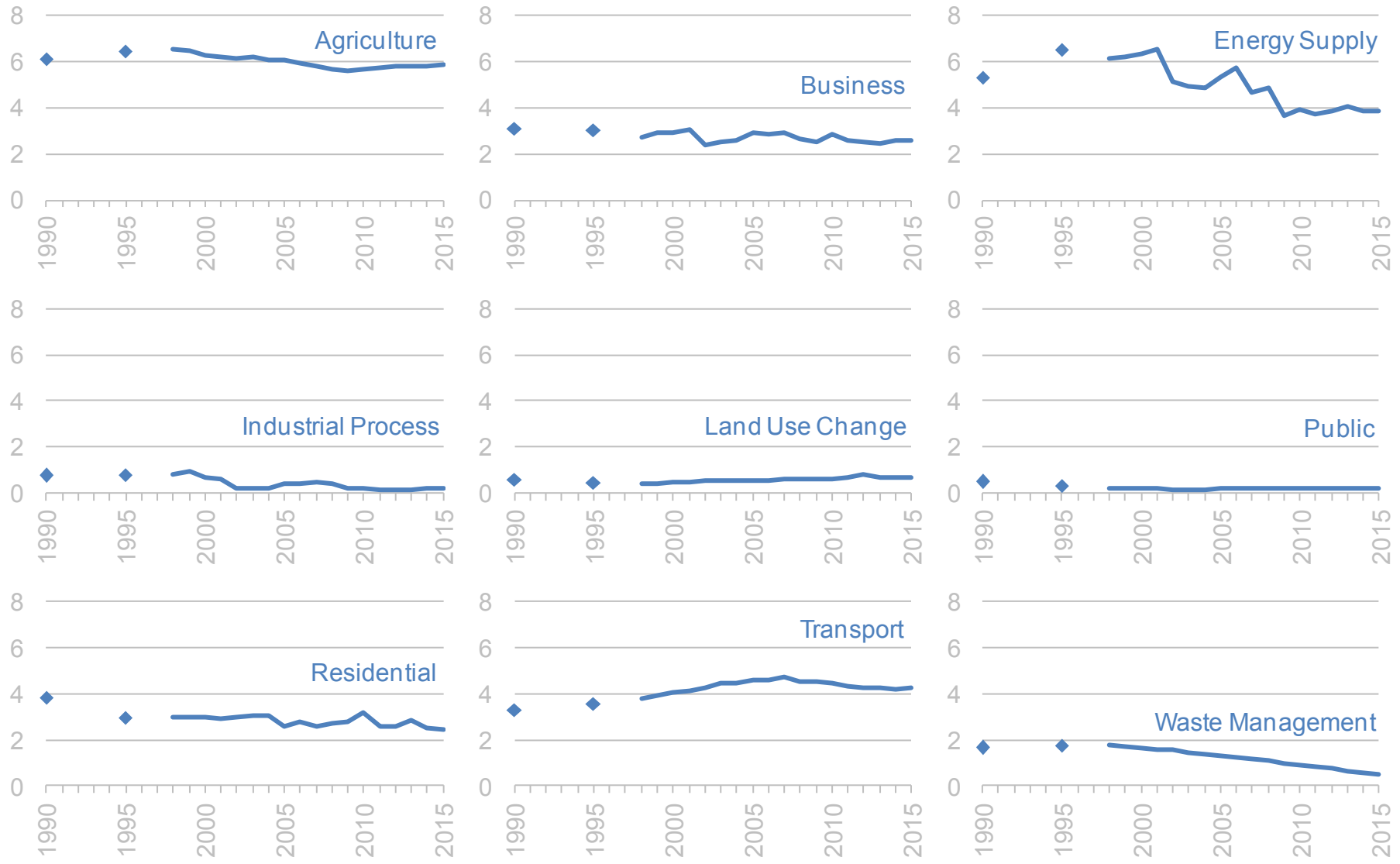
Figure 3: Greenhouse gas emissions by sector Northern Ireland, 1990 to 2015
